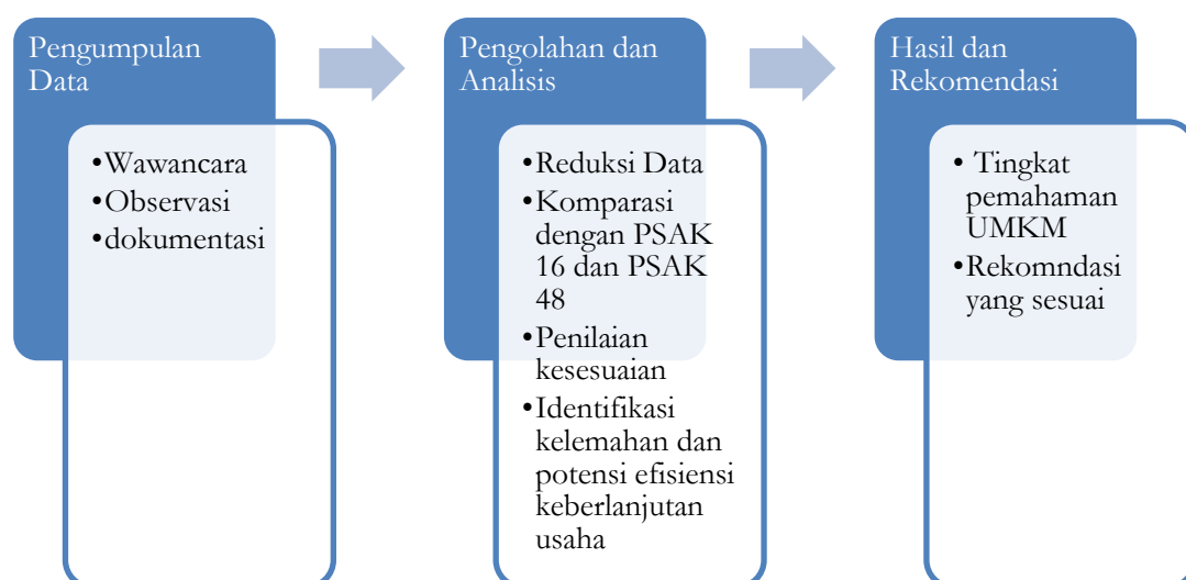
Gambar 1. Flowchart Penelitian
